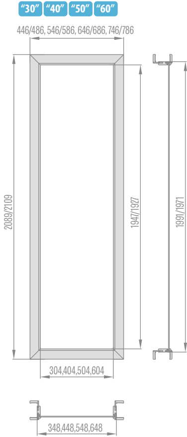
Side lights for rebated adjustable door frame strip 6cm /strip 8cm
