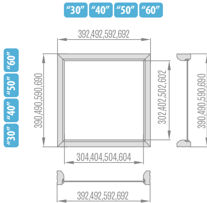
Corner lights for fixed door frame
