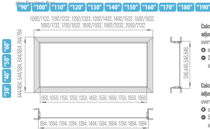
Top lights for adjustable door frame in rebated double-leaf doors
