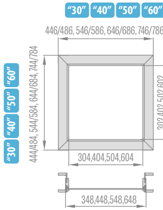
Top lights for adjustable door frame in rebated double-leaf doors
