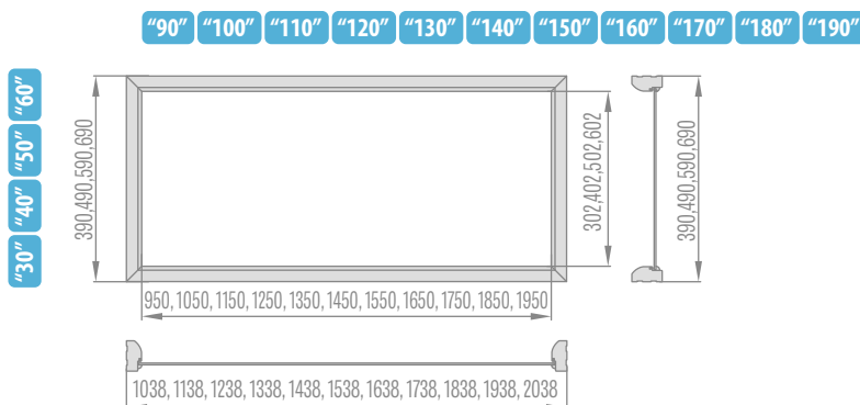
Top lights for fixed door frame in double-leaf doors
