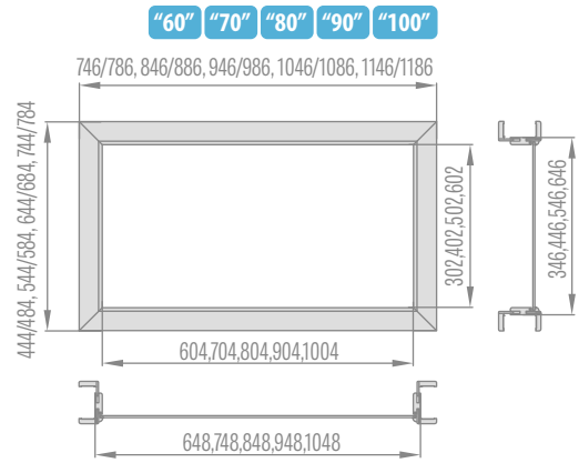
Top lights for rebated adjustable door frame in single leaf doors, 6 cm/8 cm strip
