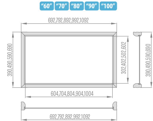
Top lights for fixed door frame in single leaf doors
