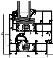
opening window - cross-section
