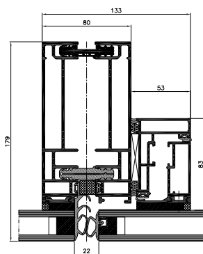
mullion and casement window - cross-section
