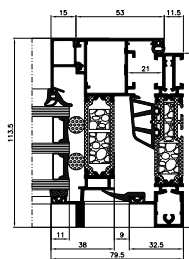
opening window - cross section
