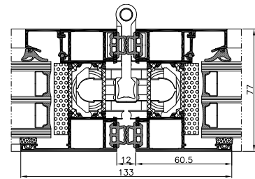
door/leaves, view
