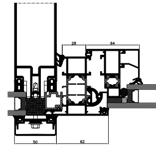
active window in a curtain wall - cross-section
