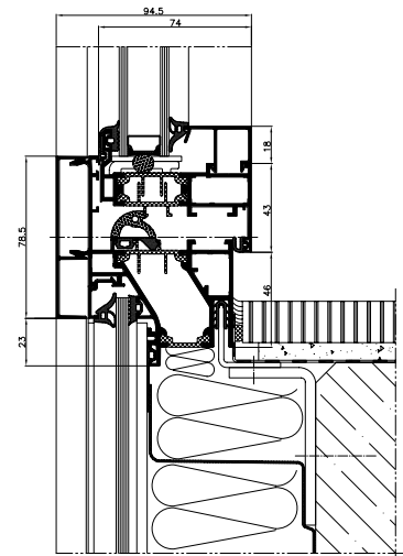
cross-section of an active window
