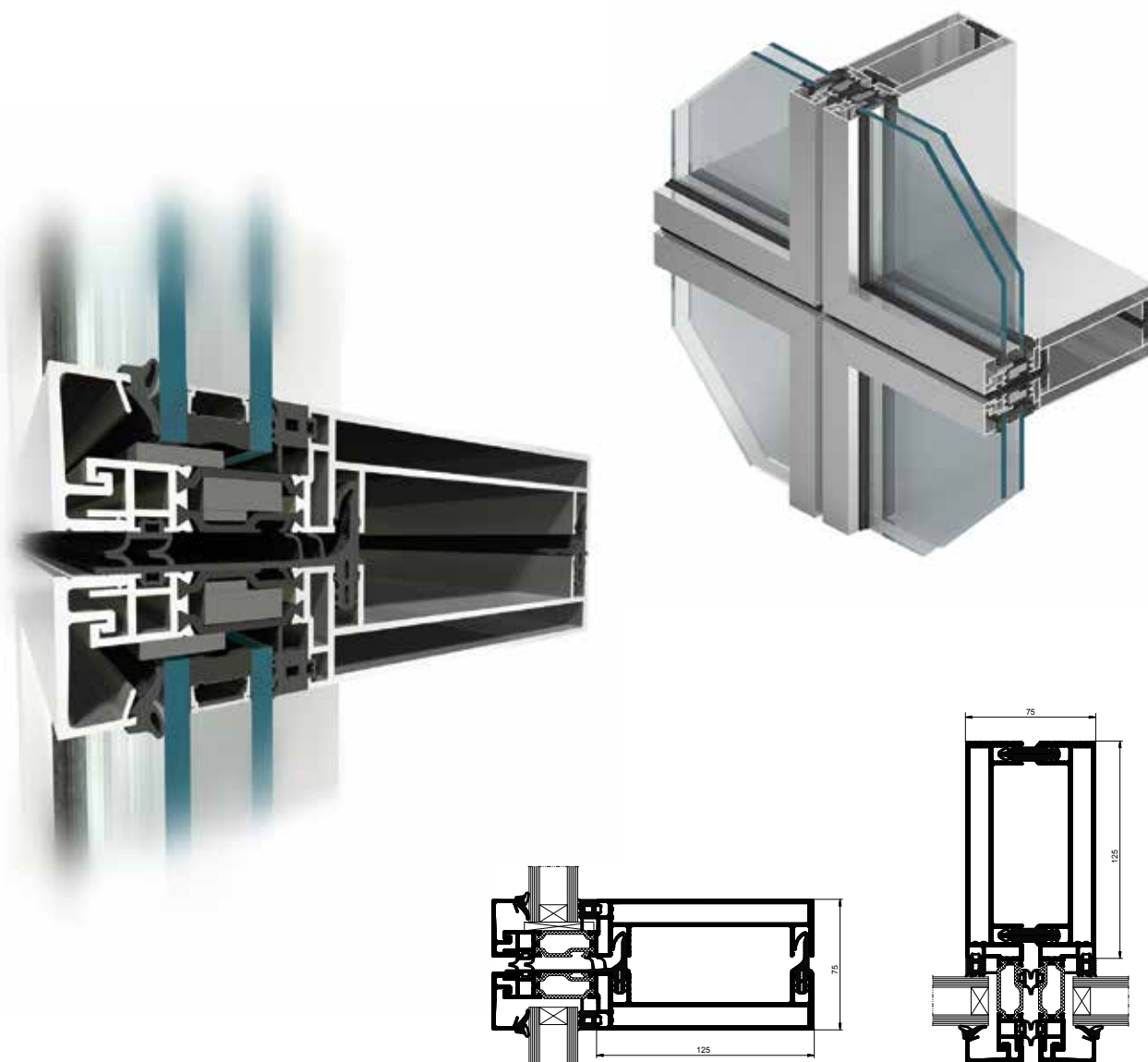
transom – cross-section
