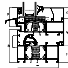
MB-70HI Window – cross-section
