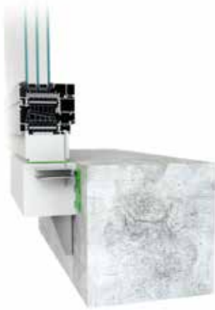
bottom connection, 100 mm beam with external anchor
