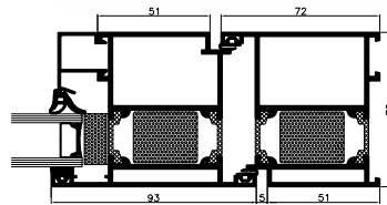
MB-70HI Door – cross-section
