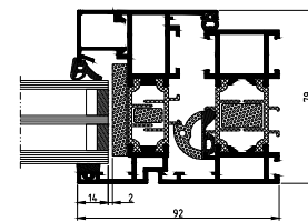
MB-70B Window – cross section
